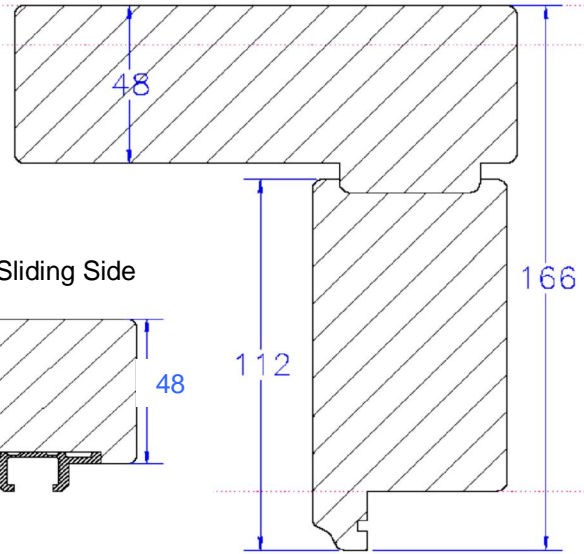
Fixed Leaf Jamb Stile 149
