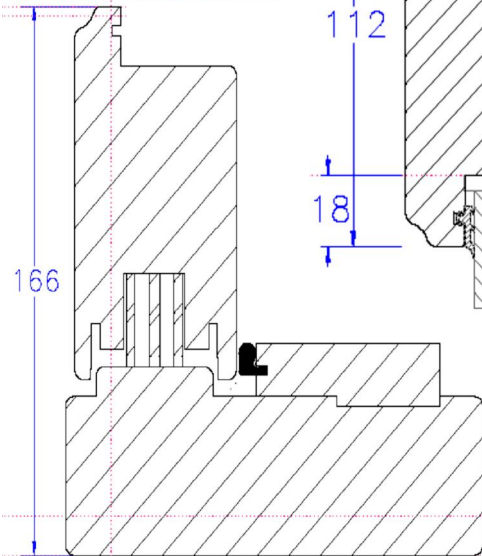
Sliding Leaf Jamb Stile
