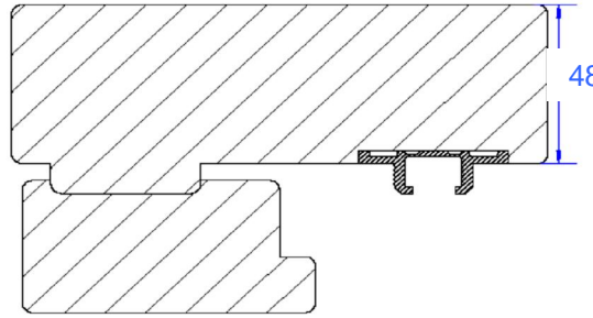
Sill detail at Sliding side
