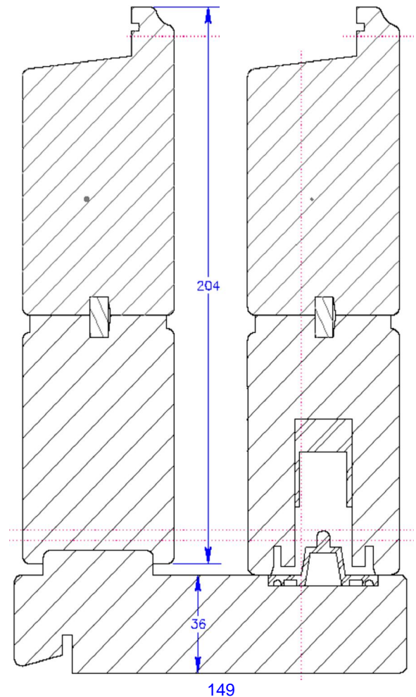
Bottom Stiles & Frame
