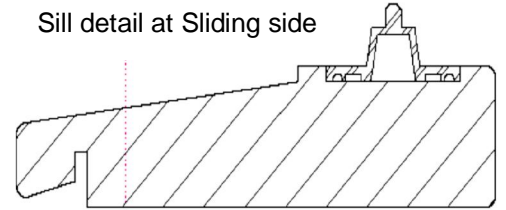
Bottom Stiles & Frame
