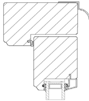
Outward folding Cill detail
