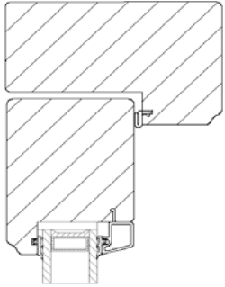
Inward folding Cill detail
