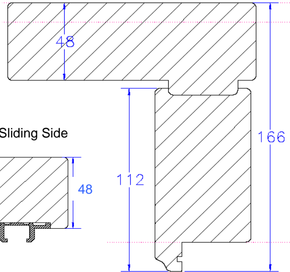
Fixed Leaf Jamb Stile 149
